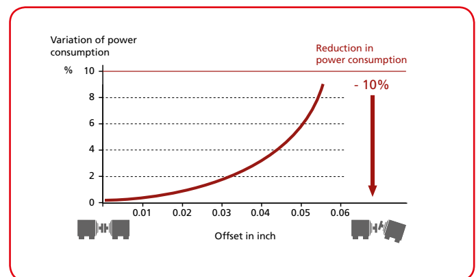
Power consumption in relation to offset. Courtesy of © ICI PLC
