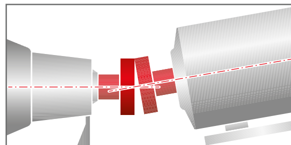
Vertical angularity
